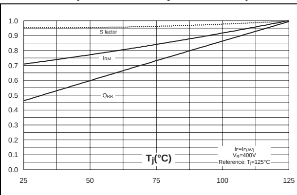
Figure 10. Relative variations of dynamic parameters vs junction temperature
