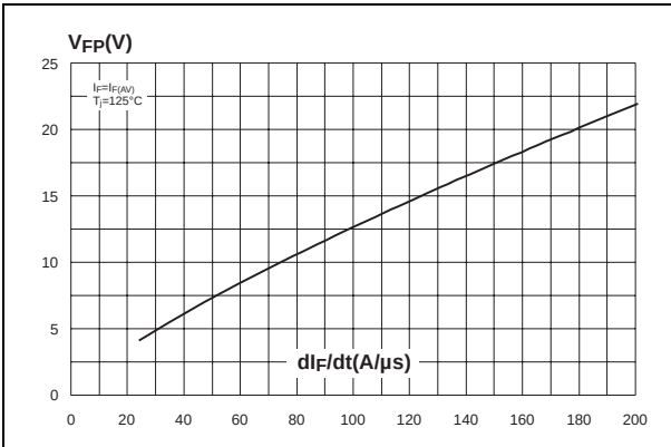
Figure 11. Transient peak forward voltage vs di_F/dt (typical values)
