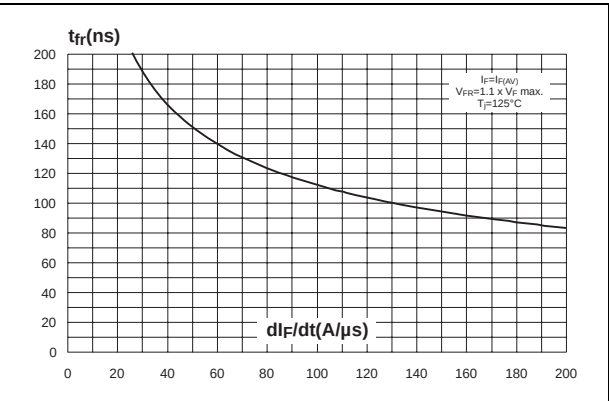
Figure 12. Forward recovery time vs di_F/dt (typical values)
