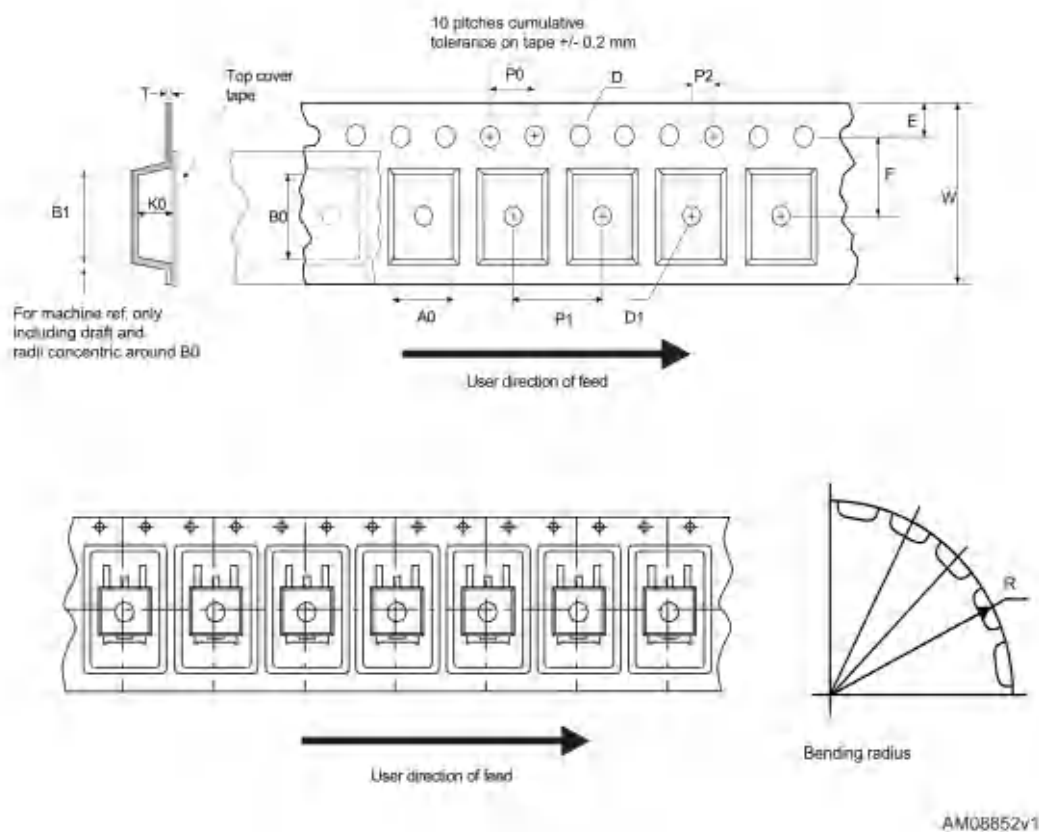
Figure 36. DPAK tape
