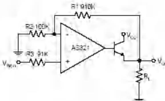
Power Amplifier
