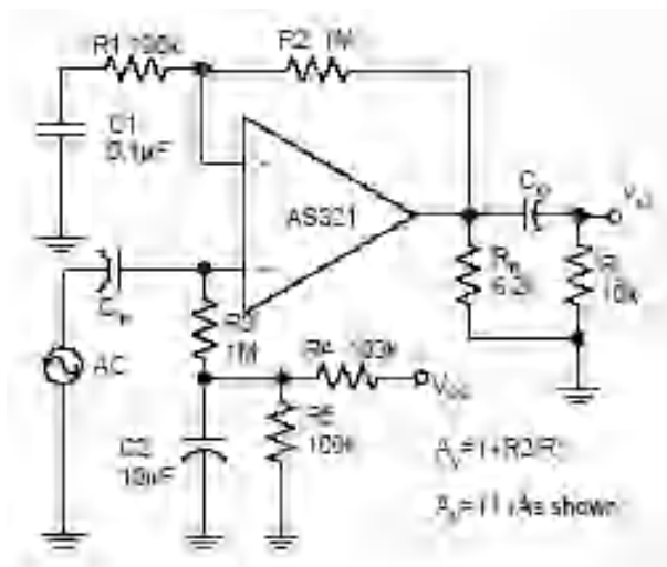
AC Coupled Non-Inverting Amplifier
