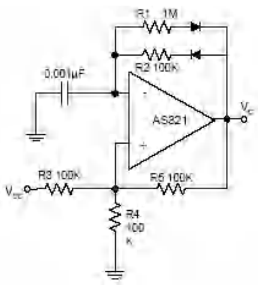
Pulse Generator
