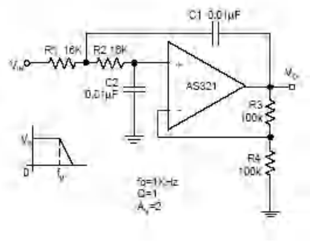
DC Coupled Low-Pass Active Filter
