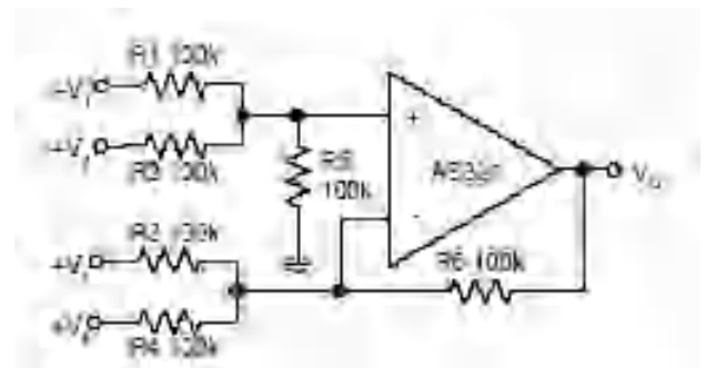
DC Summing Amplifier
