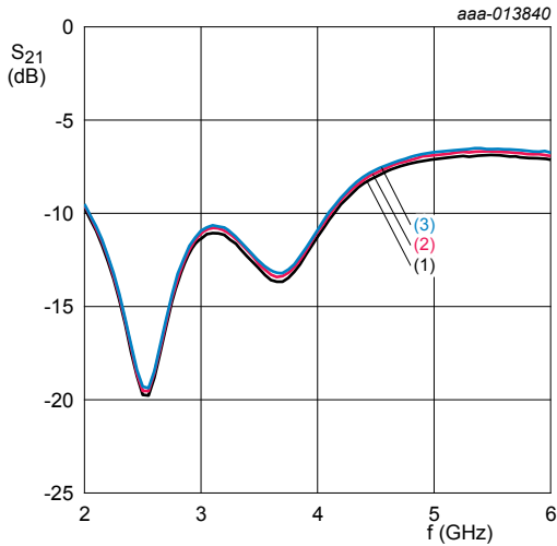
T_{amb} = 25\text{ }^{\circ}\text{C} ; V_{I(CTRL)} = 0\text{ V} ; bypass mode 1. V_{CC} = 3.0\text{ V} 2. V_{CC} = 3.3\text{ V} 3. V_{CC} = 3.6\text{ V} Figure 17. Forward transmission coefficient as a function of frequency at different supply voltages
