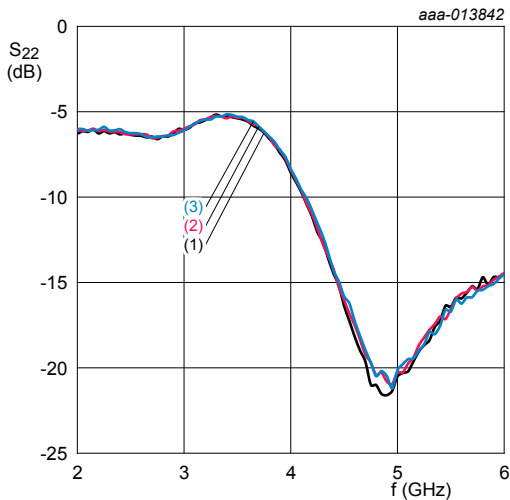
T_{amb} = 25\text{ }^{\circ}\text{C} ; V_{I(CTRL)} = 0\text{ V} ; bypass mode 1. V_{CC} = 3.0\text{ V} 2. V_{CC} = 3.3\text{ V} 3. V_{CC} = 3.6\text{ V} Figure 19. Output reflection coefficient as a function of frequency at different supply voltages
