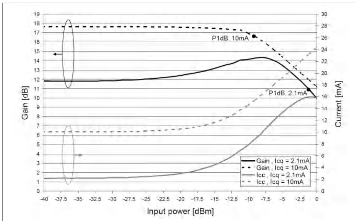
Figure 14 Power gain G = f(P_{RFin}) and supply current I_{cc} = f(P_{RFin}) at frequency f = 3.5 GHz, I_{cq} = parameter
