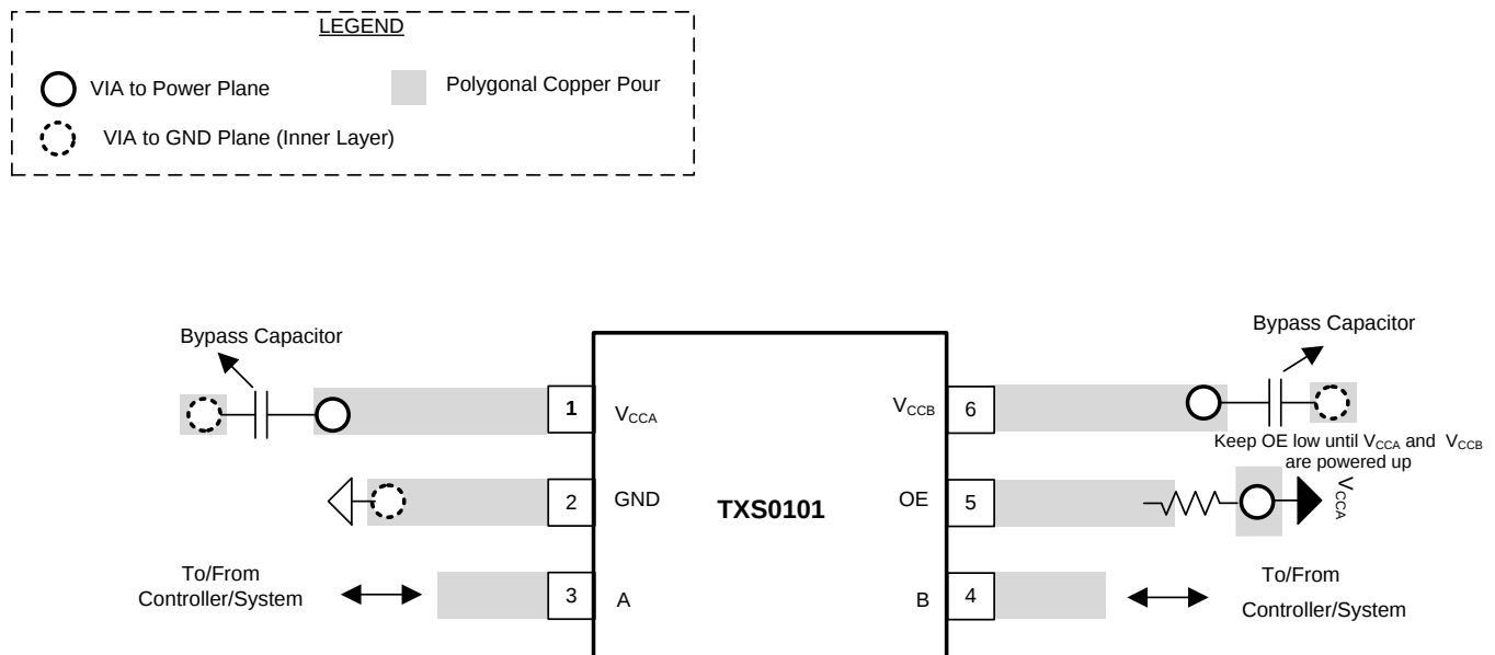
Figure 13. Typical Layout of TXS0101
