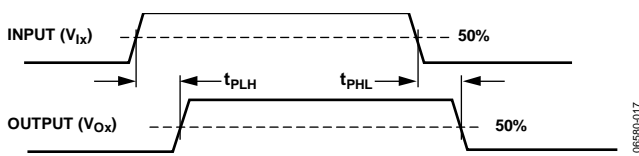
Figure 17. Propagation Delay Parameters
