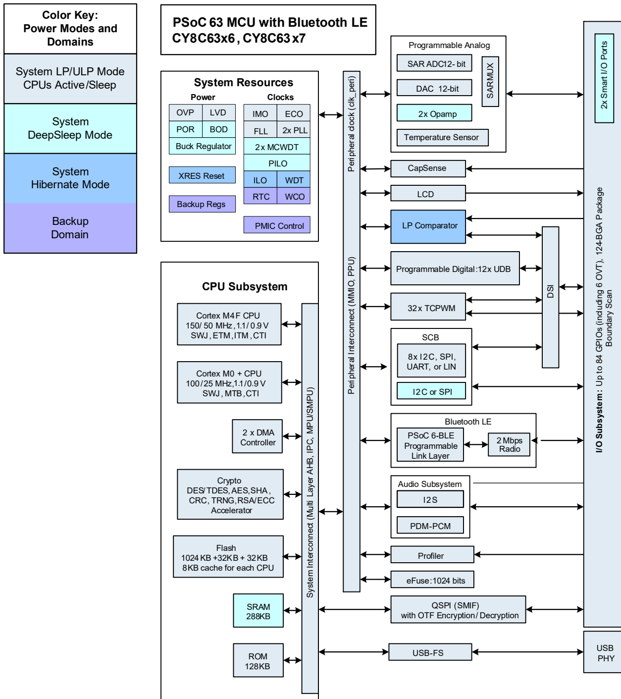
Figure 3. Block Diagram
